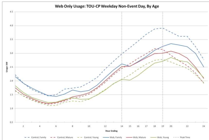
Figure 4-12 TOU-CP weekday non-event day, Web, by age
