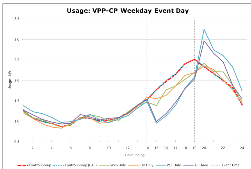
Figure 4-11 VPP-CP weekday event day, all rate-technology combinations
