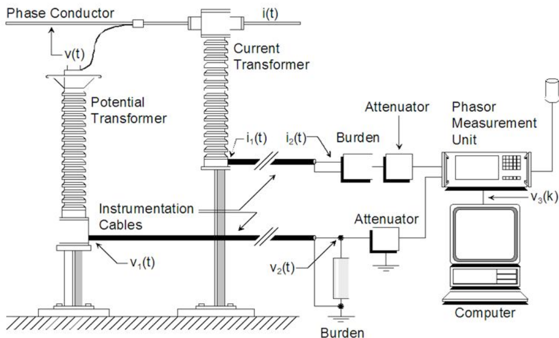
Figure 3-1 — PMU Installation
