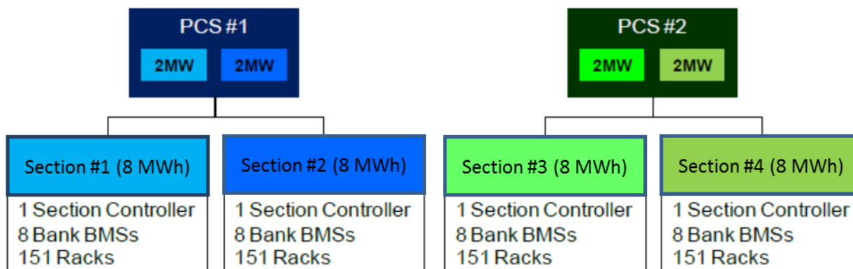
Figure 3-2 System Overview
