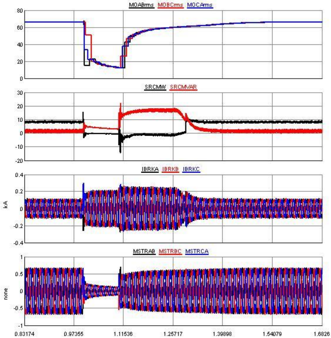
Figure 9-23 Bus Voltage, Power, and Interconnection Current and Voltage
