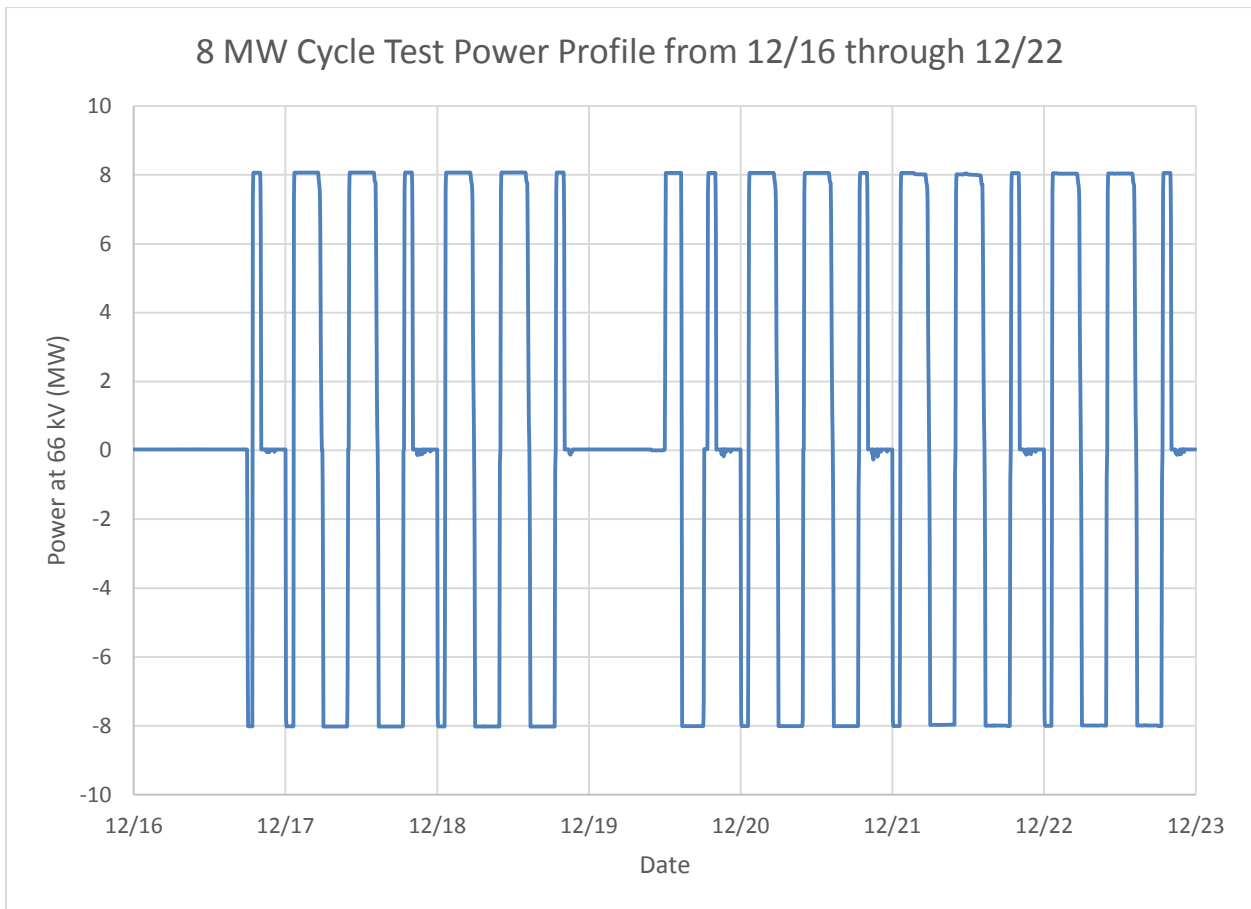
Figure 6-1 8 MW Cycle Test Power Profile from 12/16 through 12/22
