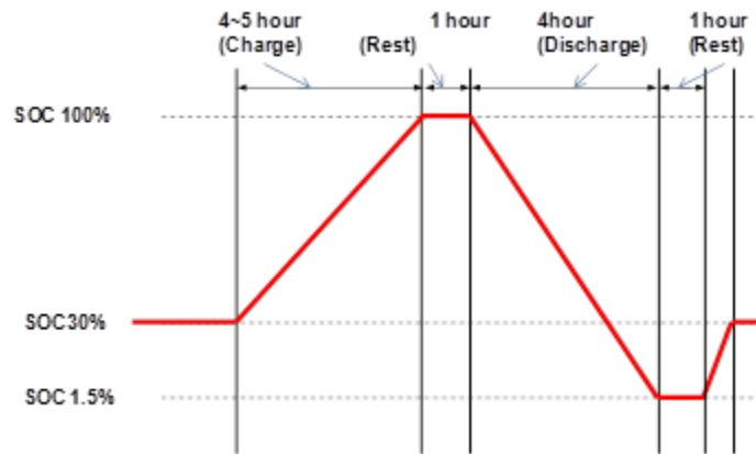
Figure 35, BESS Capacity Charge and Discharge Profile
