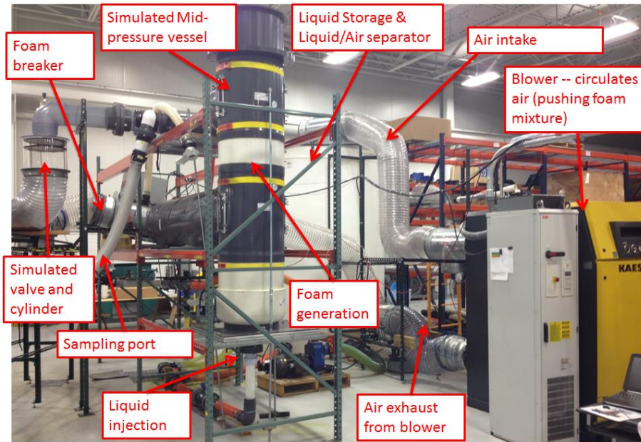
Figure 11: Foam generation and transport test stand, which mimics the mid-pressure vessel in our 1.5 MW ICAES system
