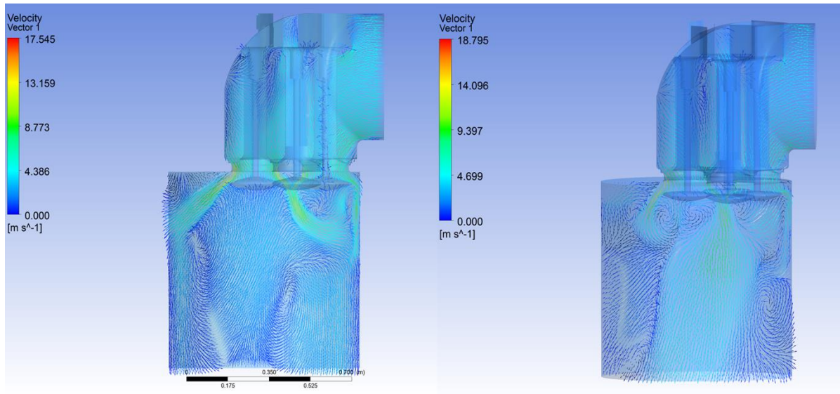
Figure 13: CFD simulation of air flow in through the low-pressure cylinder intake/exhaust valves. Left: prior to flow guide optimization, intake air forms jets that impact cylinder walls. Right: after flow guide optimization, intake flow is more uniformly distributed within cylinder.
