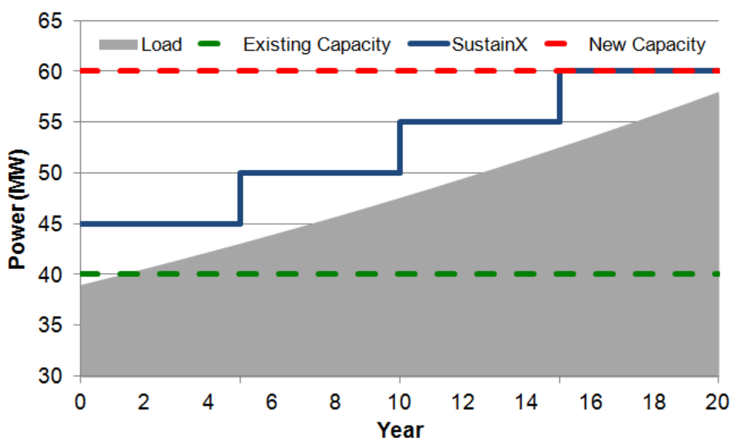
Figure 22: ICAES as a substitute for traditional grid upgrades.
