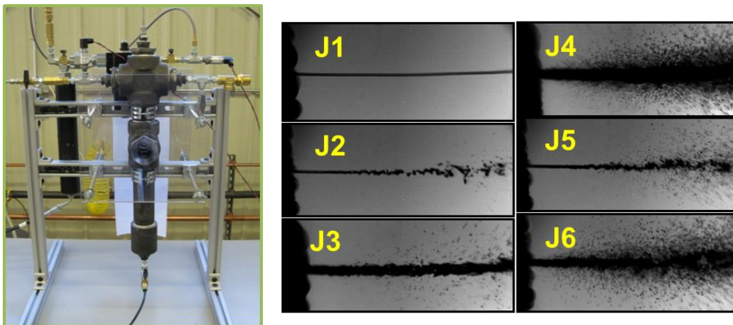
Figure 5: Spray characterization experiments. Left: HPLIA test unit. Right: jet breakup experiments using different nozzles, classified by J type per Bachalo et al.
