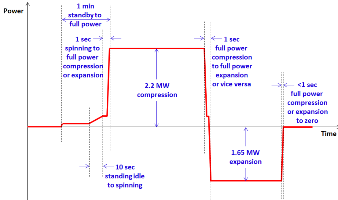
Figure 19: Illustration of system response times
