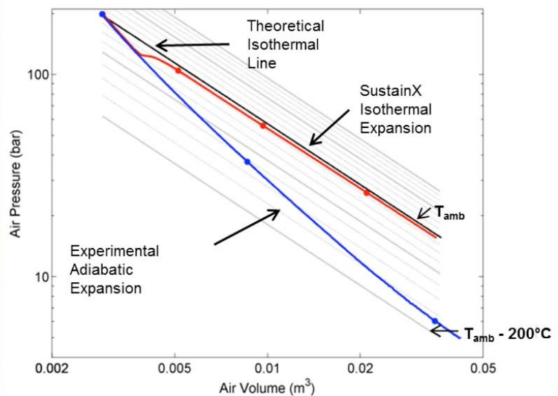
Figure 6: Left: Heat-transfer test stand, a.k.a. HXTST. Right: Experimental results for an isothermal expansion (red) vs. adiabatic expansion (blue) vs ideal expansion (black) for the same mass of air. Dots are marked at 1 second intervals for reference. Grey lines are lines of constant temperature at 25°C increments from ambient temperature.
