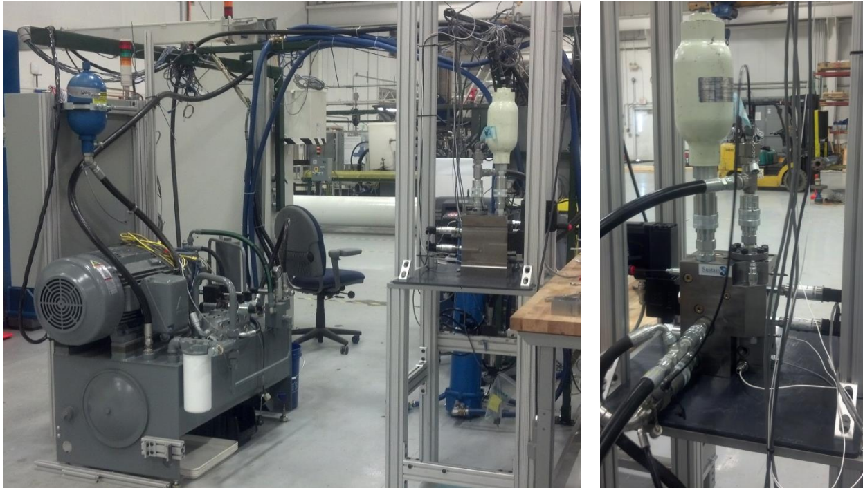
Figure 14: Valve actuator test stand. Left: Full test stand showing hydraulic power unit and control cabinet at left and test table at right. Right: close-up of valve actuator on test table
