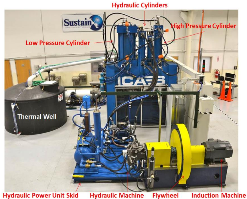
Figure 8: 40 kW Pilot unit, with major components identified, after the move to Seabrook, NH
