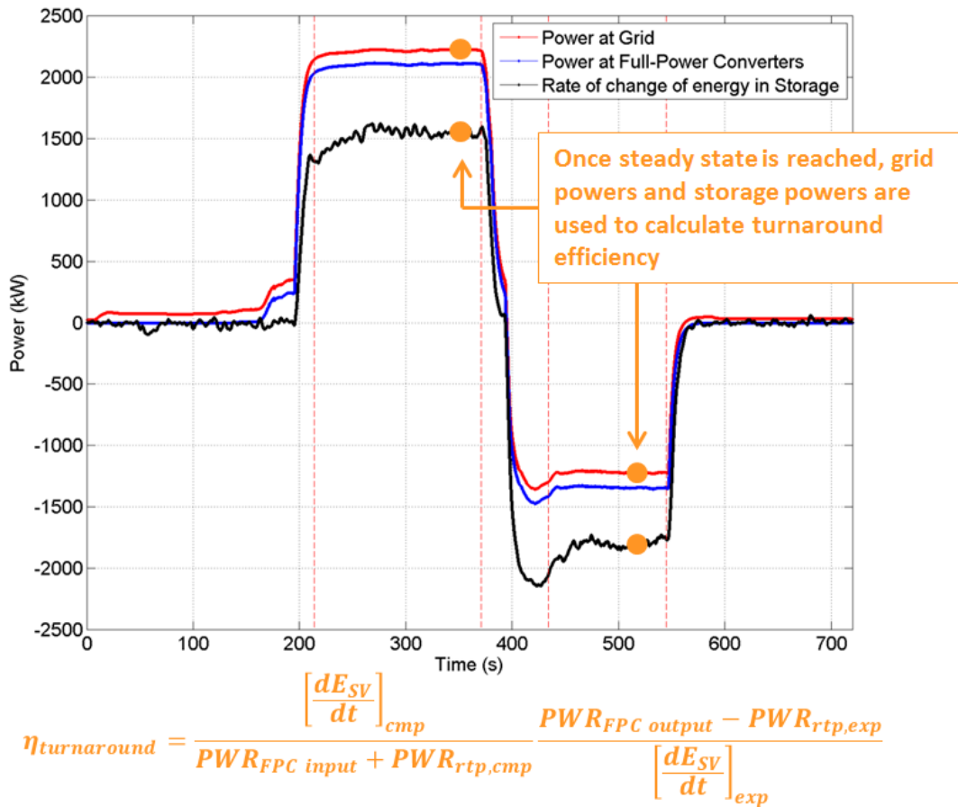
Figure 17: Plot of experimentally measured grid power and “storage power”, illustrating the calculation of turnaround efficiency. A description of abbreviations is shown in Table 4.
