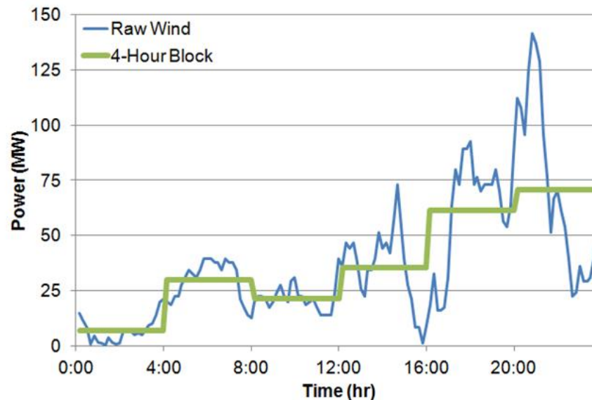
Figure 21: Multi-hour firm wind with ICAES.
