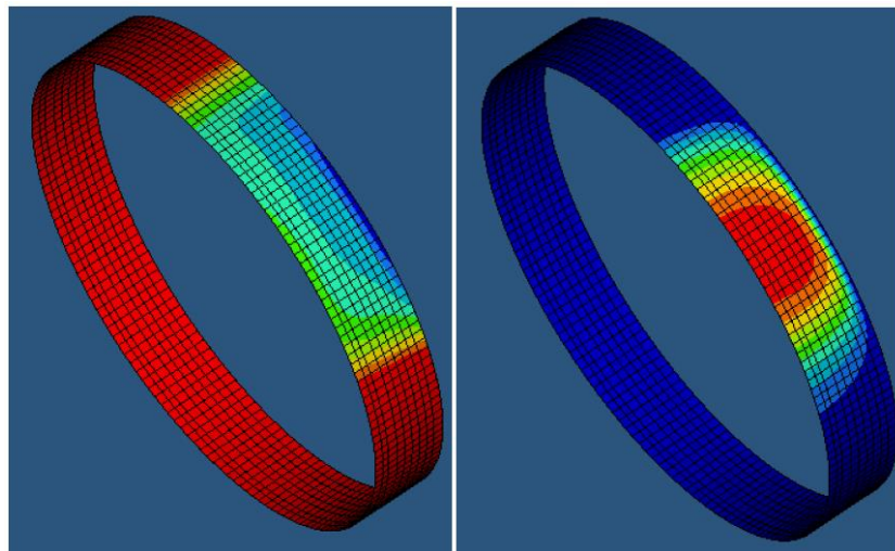
Figure 12: Dynamic elasto-hydrodynamic simulation results from MAN for the crank-pin bearing of the high-pressure cylinder at top dead center. Left: oil film thickness. Right: oil film pressure.
