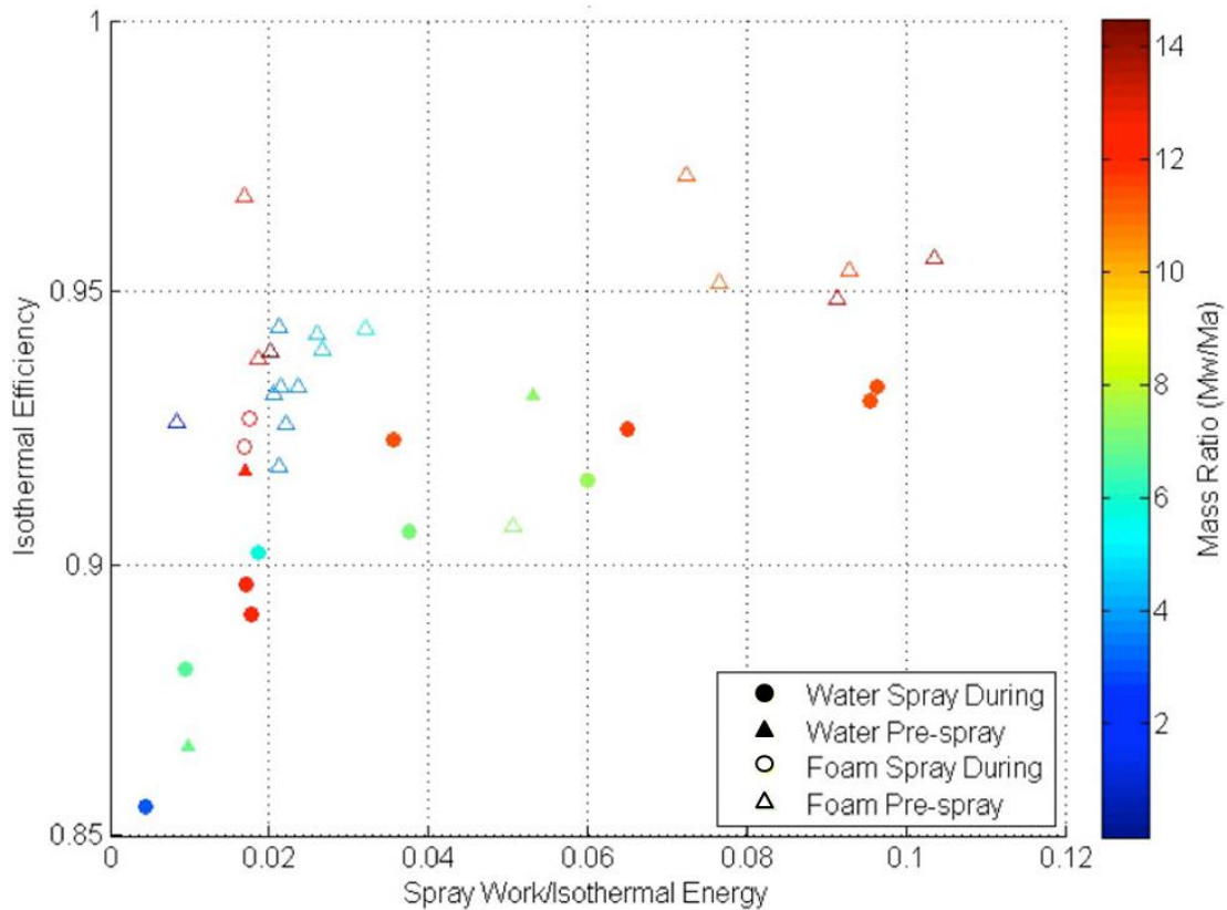
Figure 10: Data on spray and foam heat transfer from air expansions at the same power levels in a SustainX heat-transfer test stand. Foam generated before expansion (“foam pre-spray”—open triangles) achieved substantially higher efficiency at lower spray- energy (work) input levels than direct spray injection of droplets (closed circles)
