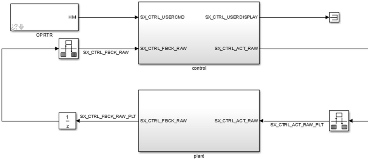
Figure 16: top-level view of the control software integrated into a closed loop with a mathematical model of the plant (full system), allowing for a priori testing and validation of the control system. (Abbreviations are SX:SustainX, CTRL: control, ACT: actuator, FBCK: feedback, CMD: command, HMI: human machine interface, OPTR: operator)
