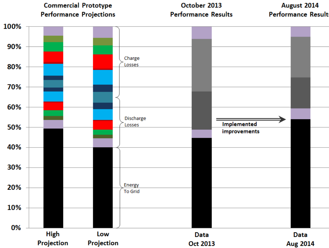
Figure 18: 1.5 MW Commercial Prototype efficiency results compared to initial projections. Color Code: Black: electricity to grid; Purple: parasitic electric; Greens: PMG and FPCs; Reds: Crank and pistons; Blues: Pneumatics; Greys: Unallocated
