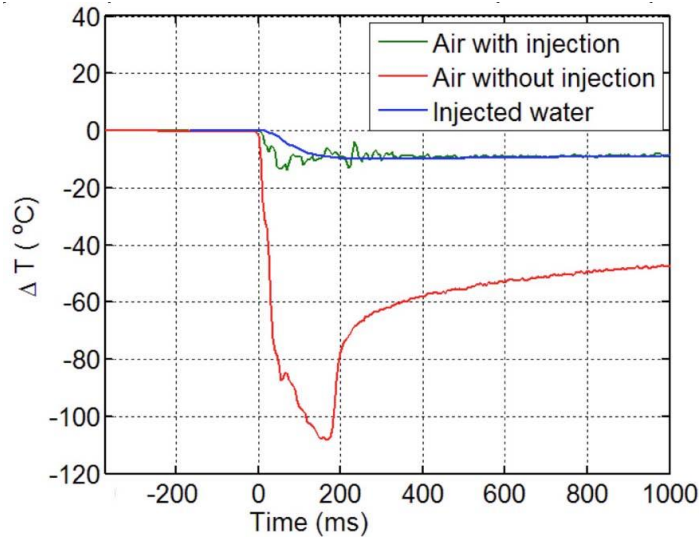
Figure 9: Comparison of non-isothermal to approximately isothermal air expansion with foam in the HXTST test cylinder: quarter-second piston stroke (0–250 ms), pressure change from ~200 bar to ~20 bar. Air temperature change ( \Delta T ) is shown without heat exchange (red) and with foam heat exchange (green). Liquid temperature (blue) decreases slightly as heat is transferred from liquid to air; liquid and air quickly achieve thermal equilibrium (i.e., approach a common temperature). Without foam, maximum temperature drop is 108°C; with foam, only 12°C.
